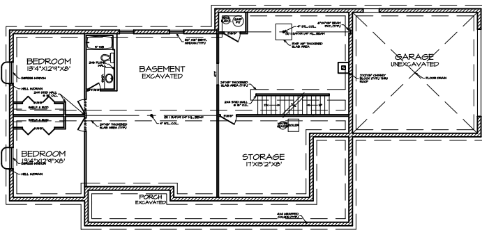
2 FOUNDATION PLAN A-2
