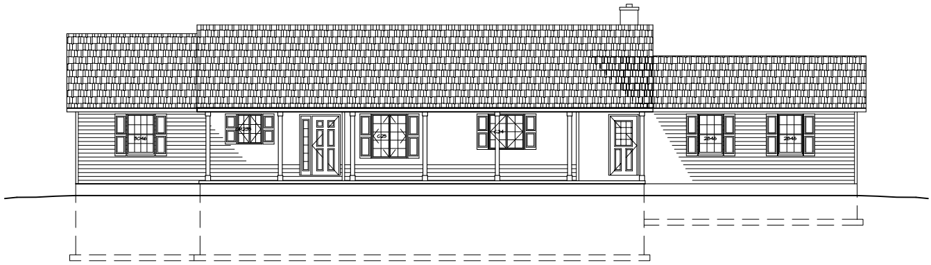
1 FRONT ELEVATION A-1
