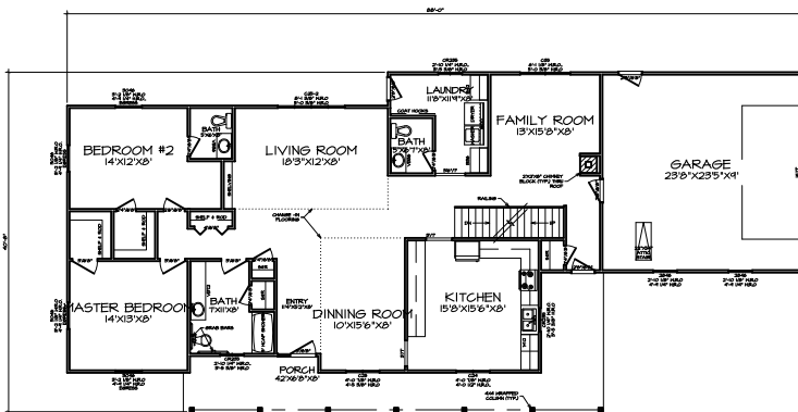
3 FIRST FLOOR PLAN A-3
